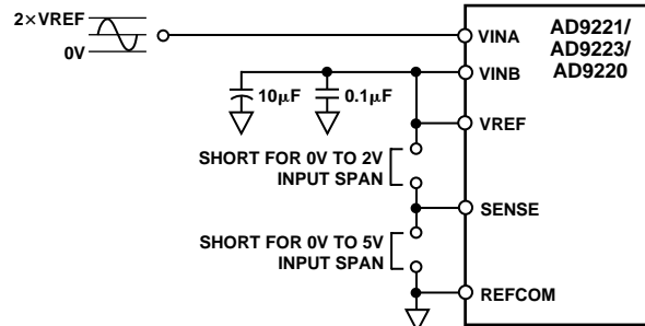
Figure 47. Internal Reference—2 V p-p Input Span, V_{CM} = 1 \text{ V} , or 5 V p-p Input Span, V_{CM} = 2.5 \text{ V}
