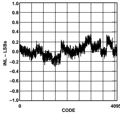
Figure 3. Typical INL
