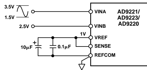
Figure 48. Internal Reference—2 V p-p Input Span, V_{CM} = 2.5 \text{ V}
