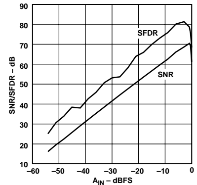
Figure 28. SNR/SFDR vs. A_{\text{IN}} (Input Amplitude) ( f_{\text{IN}} = 5.0 \text{ MHz} , Input Span = 2 V p-p, V_{\text{CM}} = 2.5 \text{ V} )
